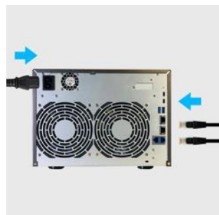
AS6808T / AS6810T
